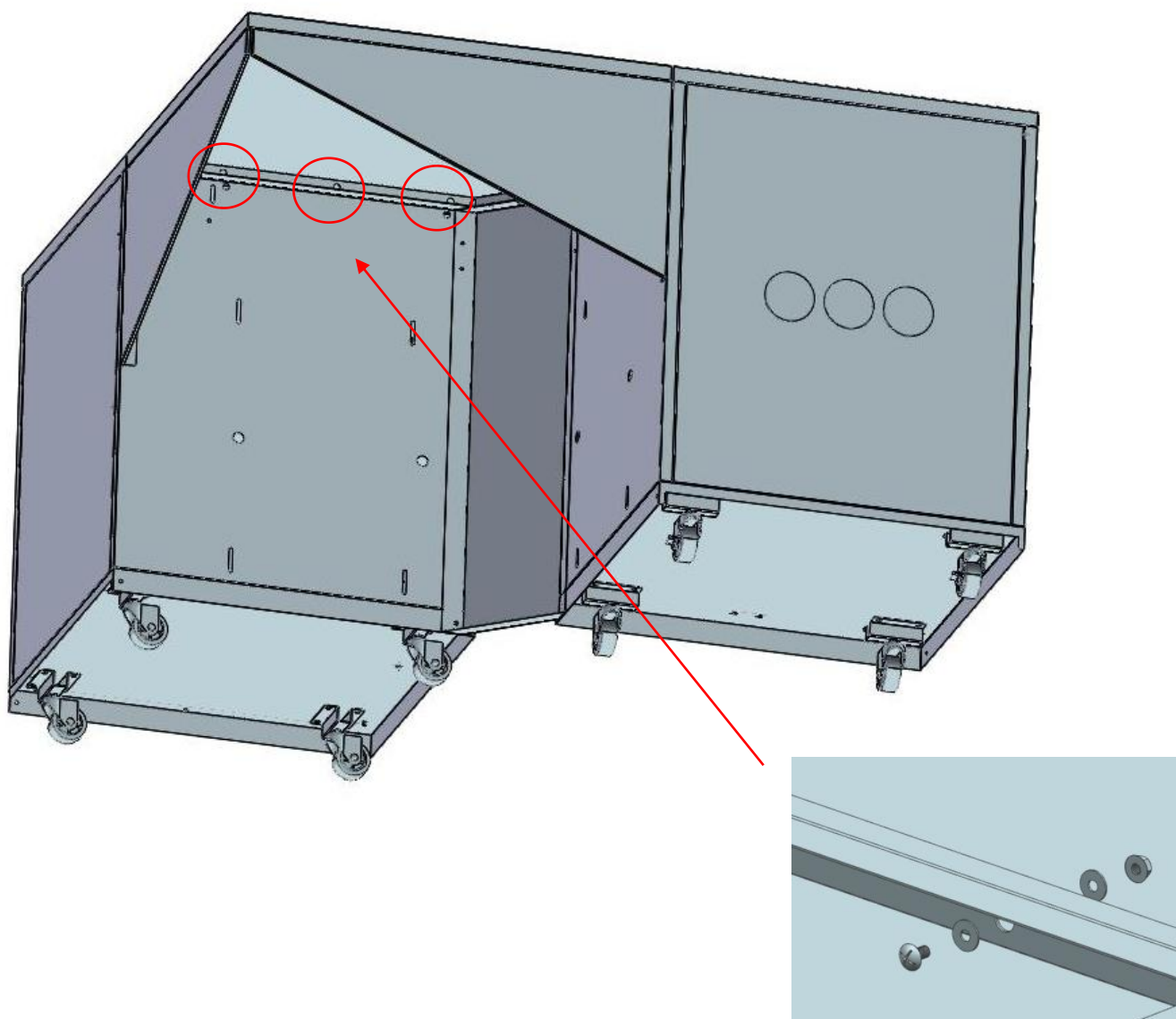
Bottom-Up View
